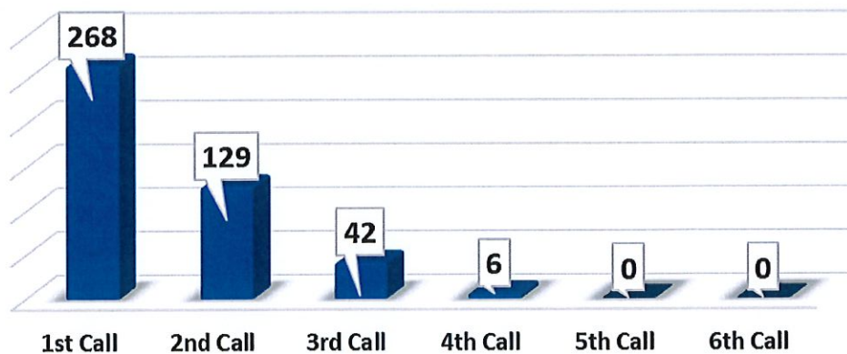
Call Sequence
